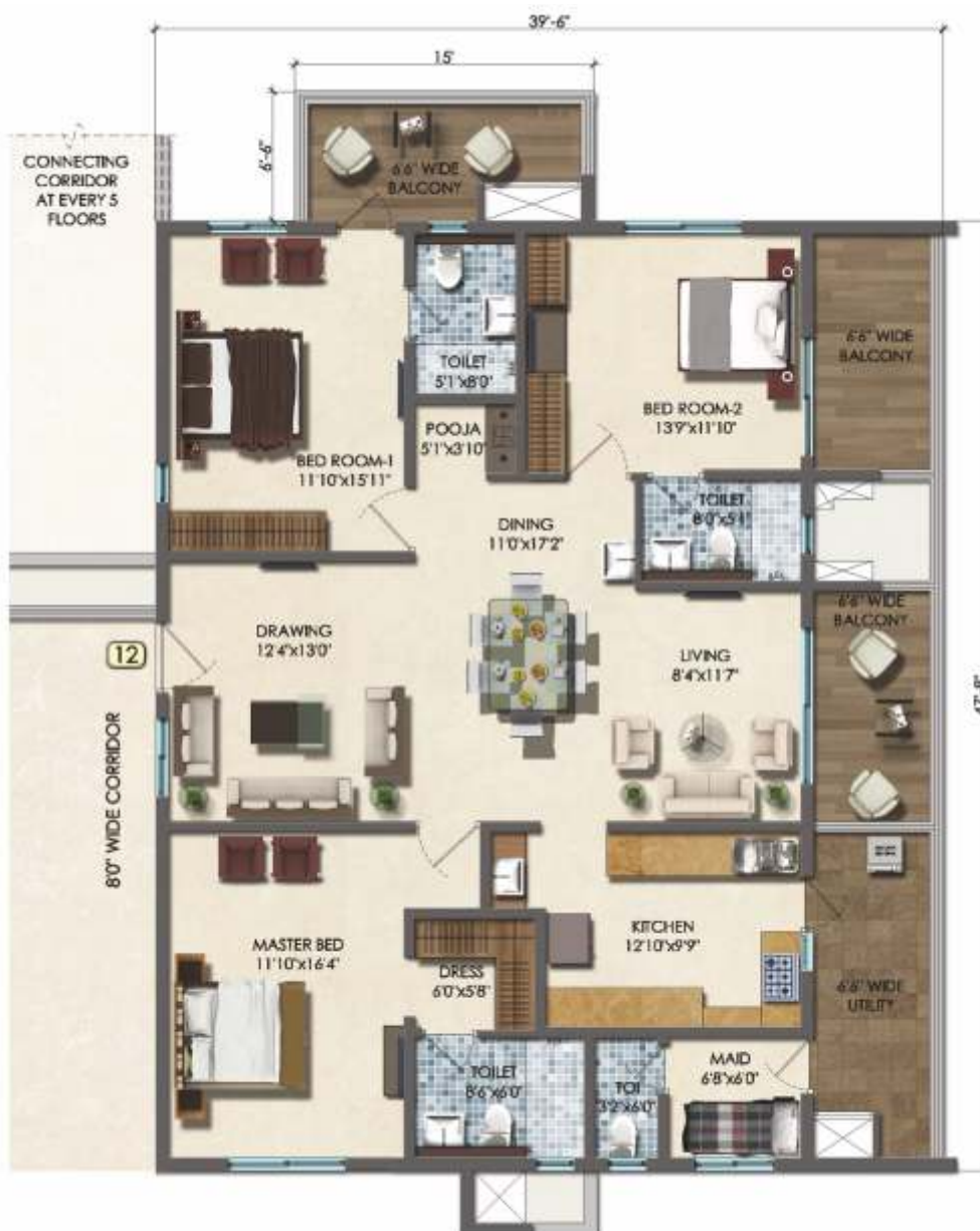
BLOCK - B TYPICAL FLOOR PLAN
